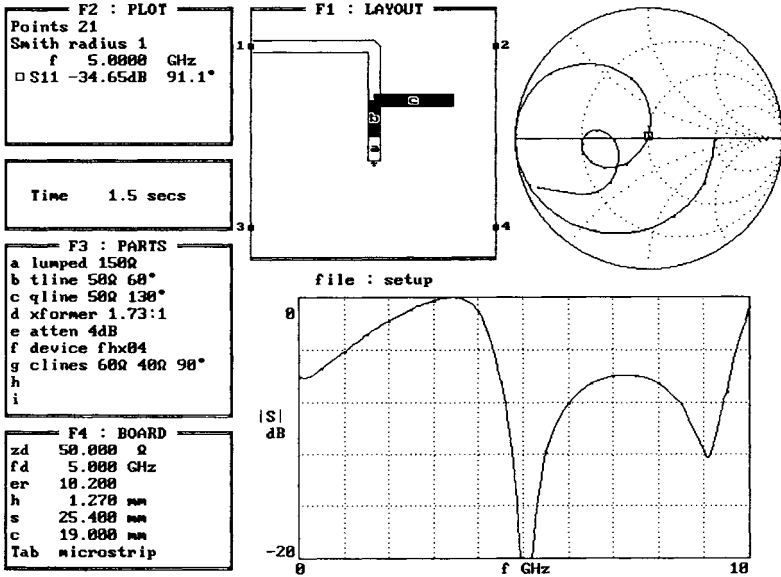
Figure 1.5 Shunt-stub matching.
